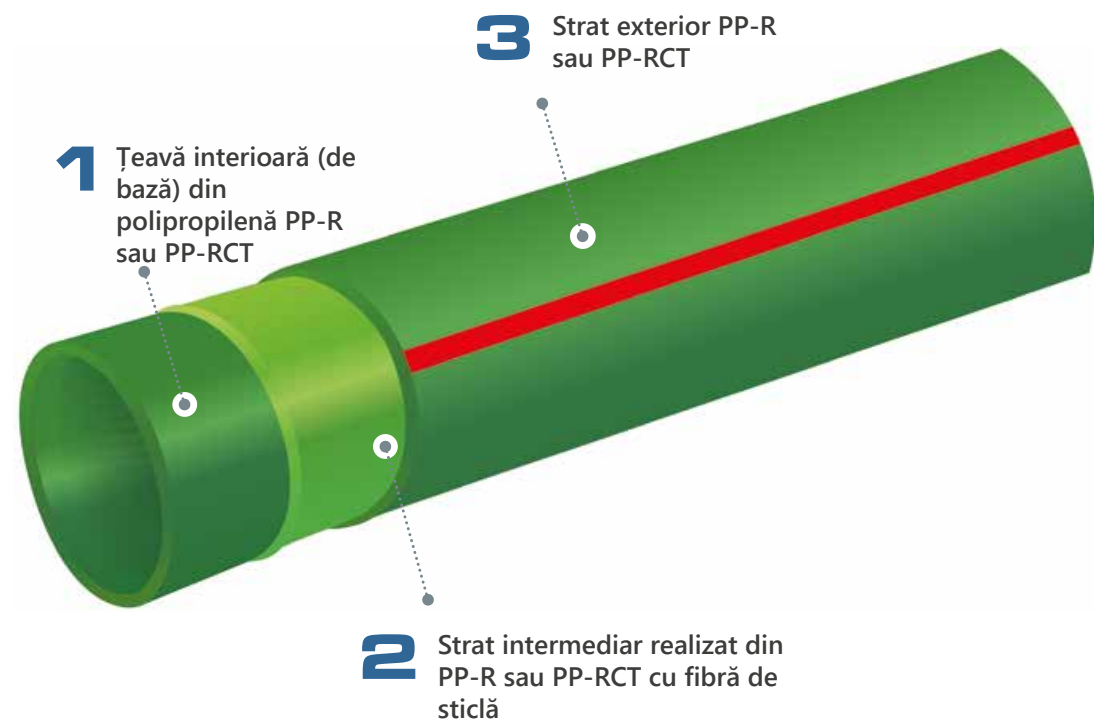
Structura țevii KAN-therm PP Glass
